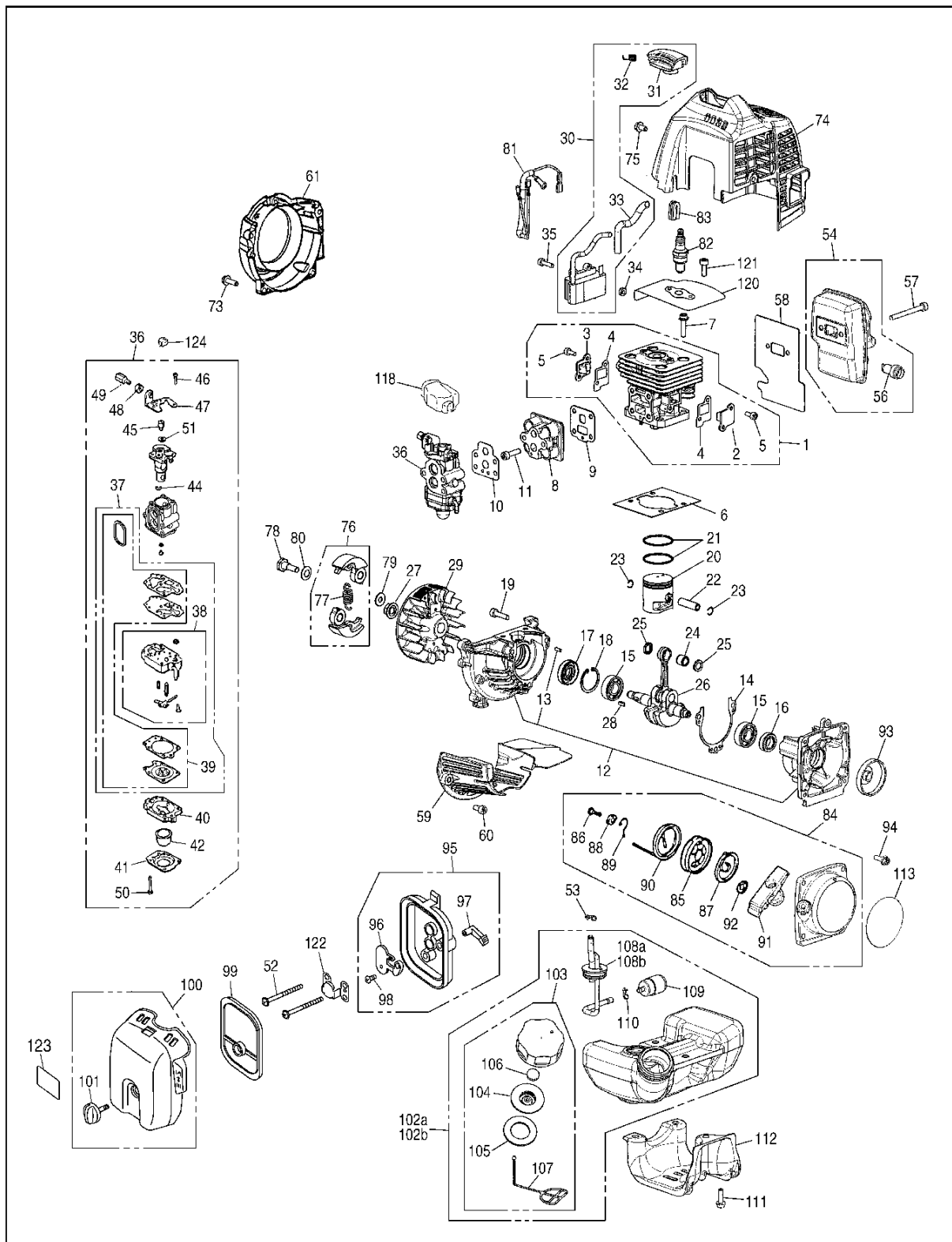
Fig.3 ENGINE UNIT
