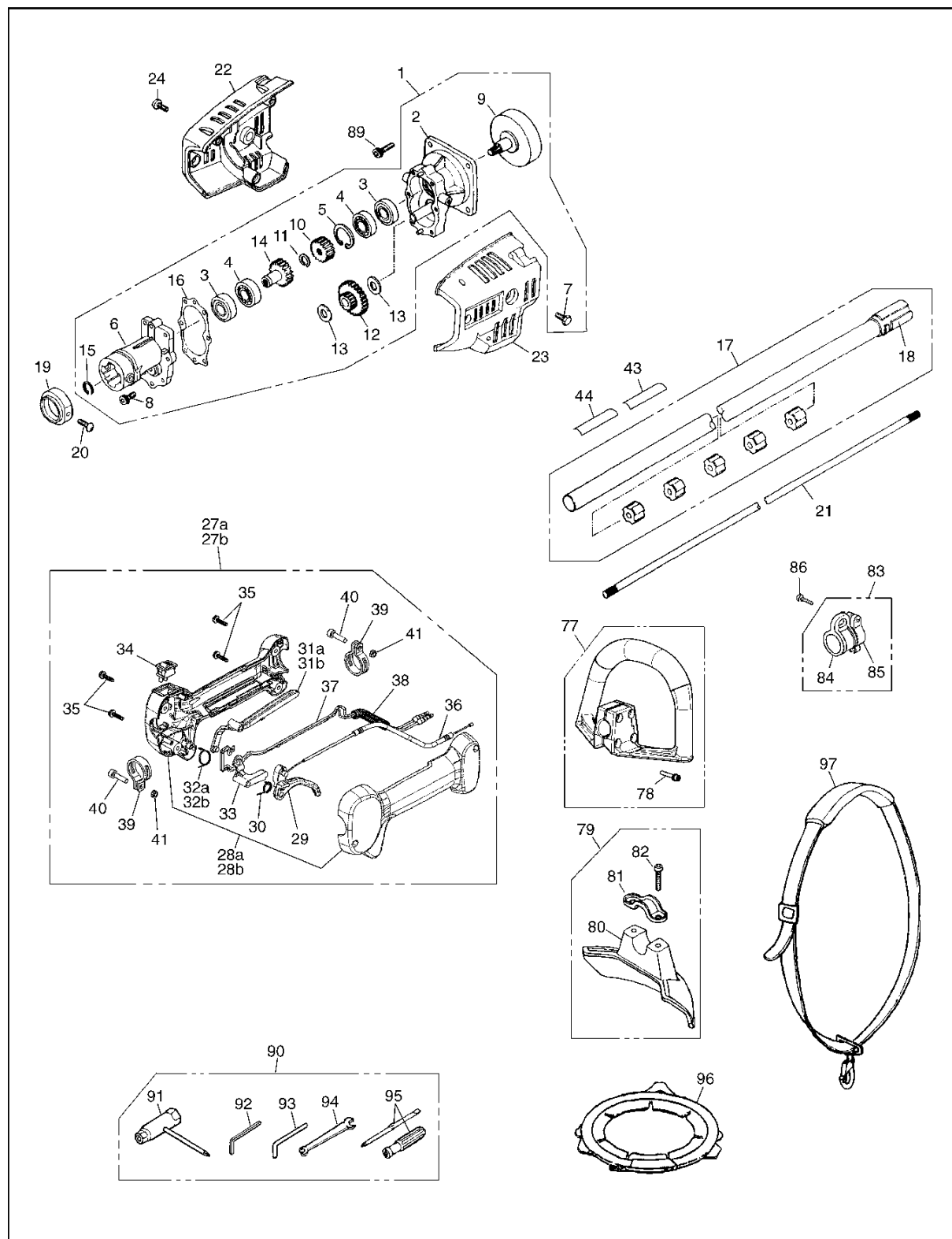
Fig.1 DRIVE UNIT
