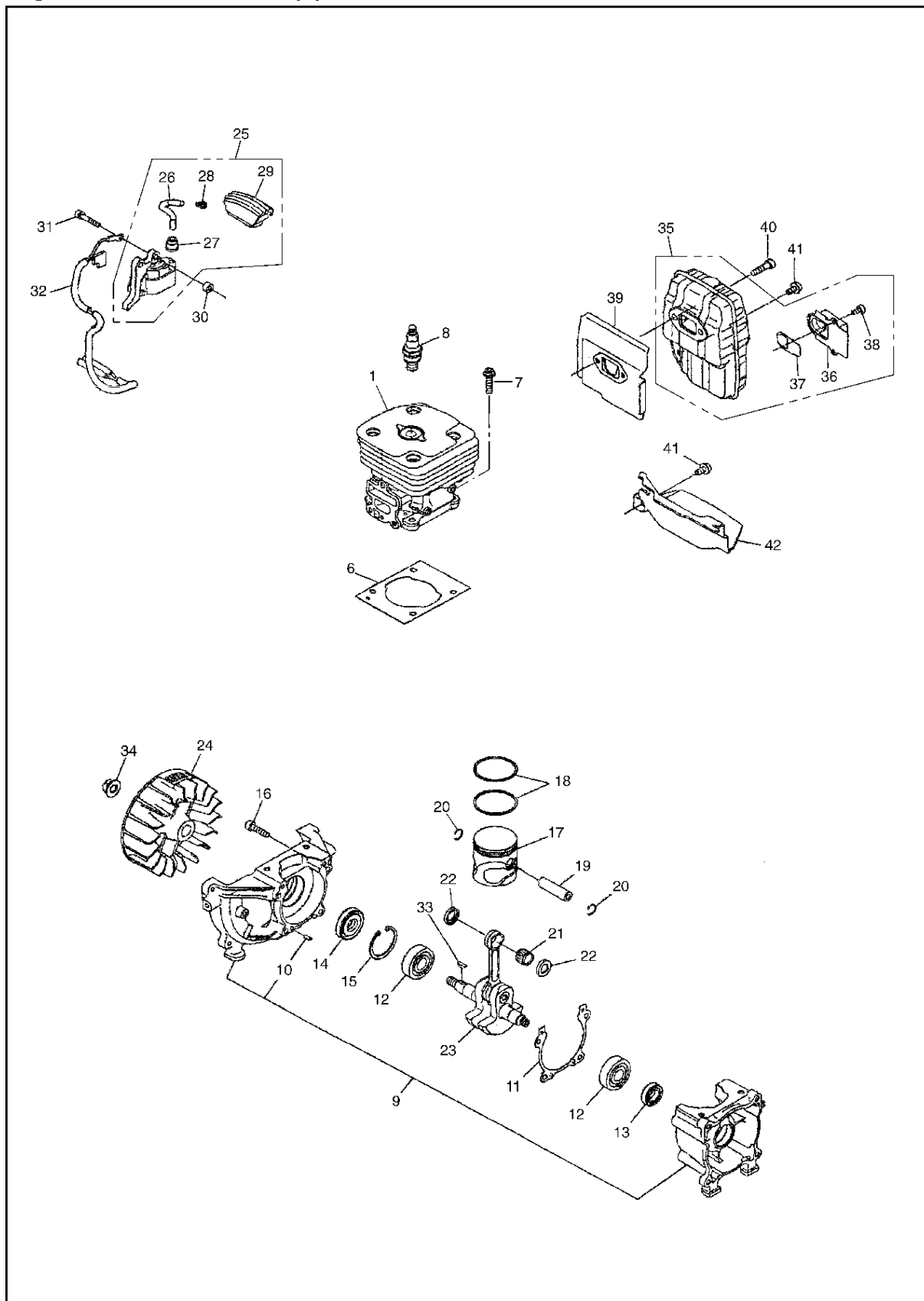
Fig.3 ENGINE GROUP (1)
