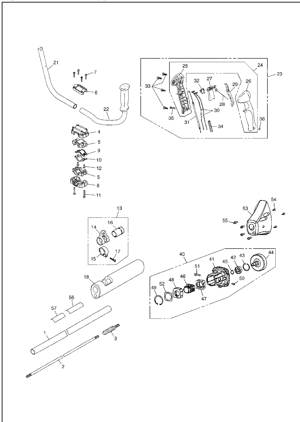
Fig.1 CUTTER GROUP (1)
