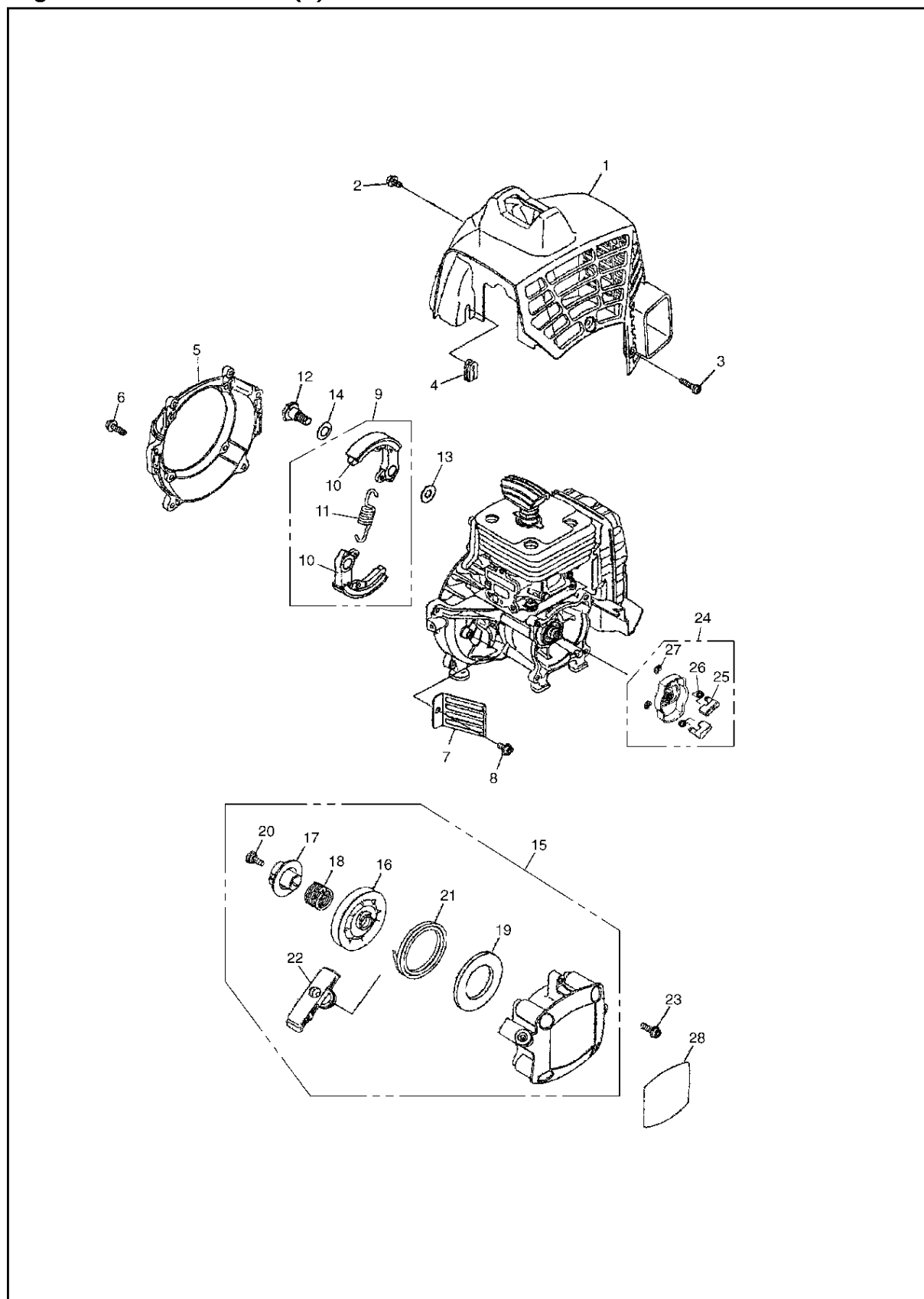
Fig.5 ENGINE GROUP (3)
