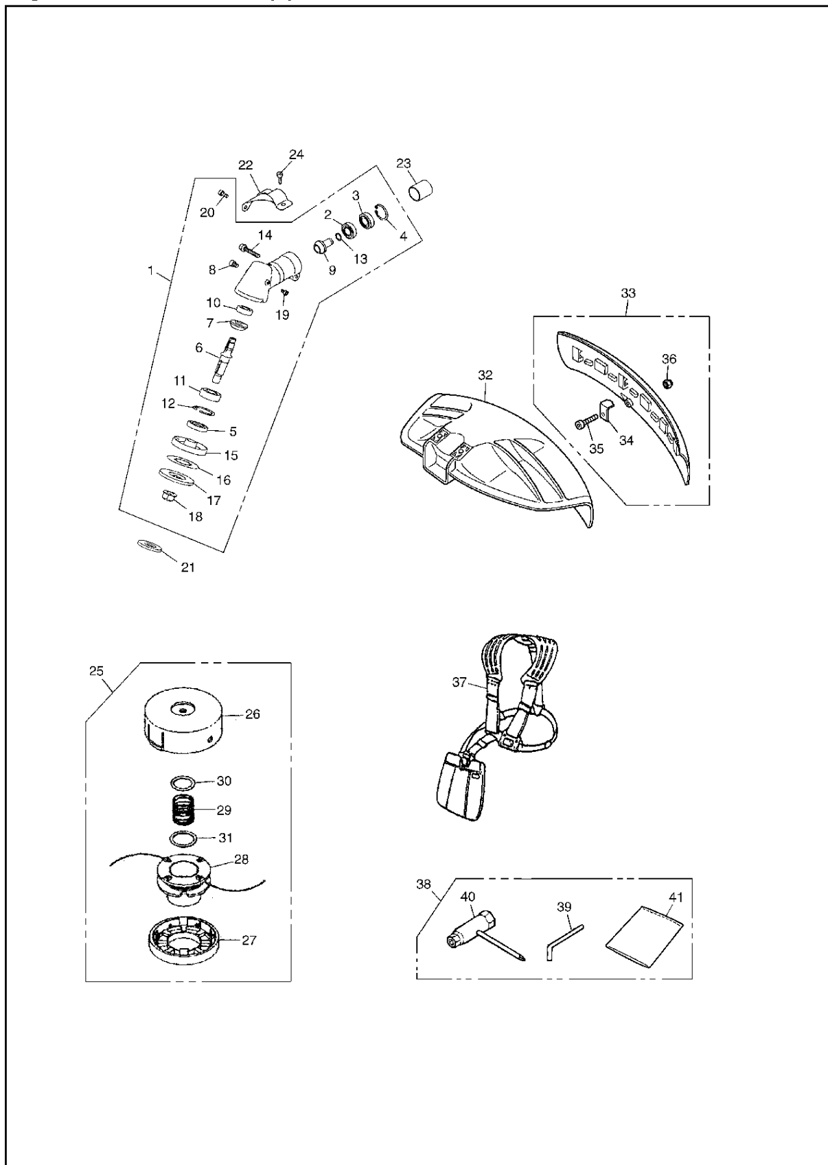
Fig.2 CUTTER GROUP (2)
